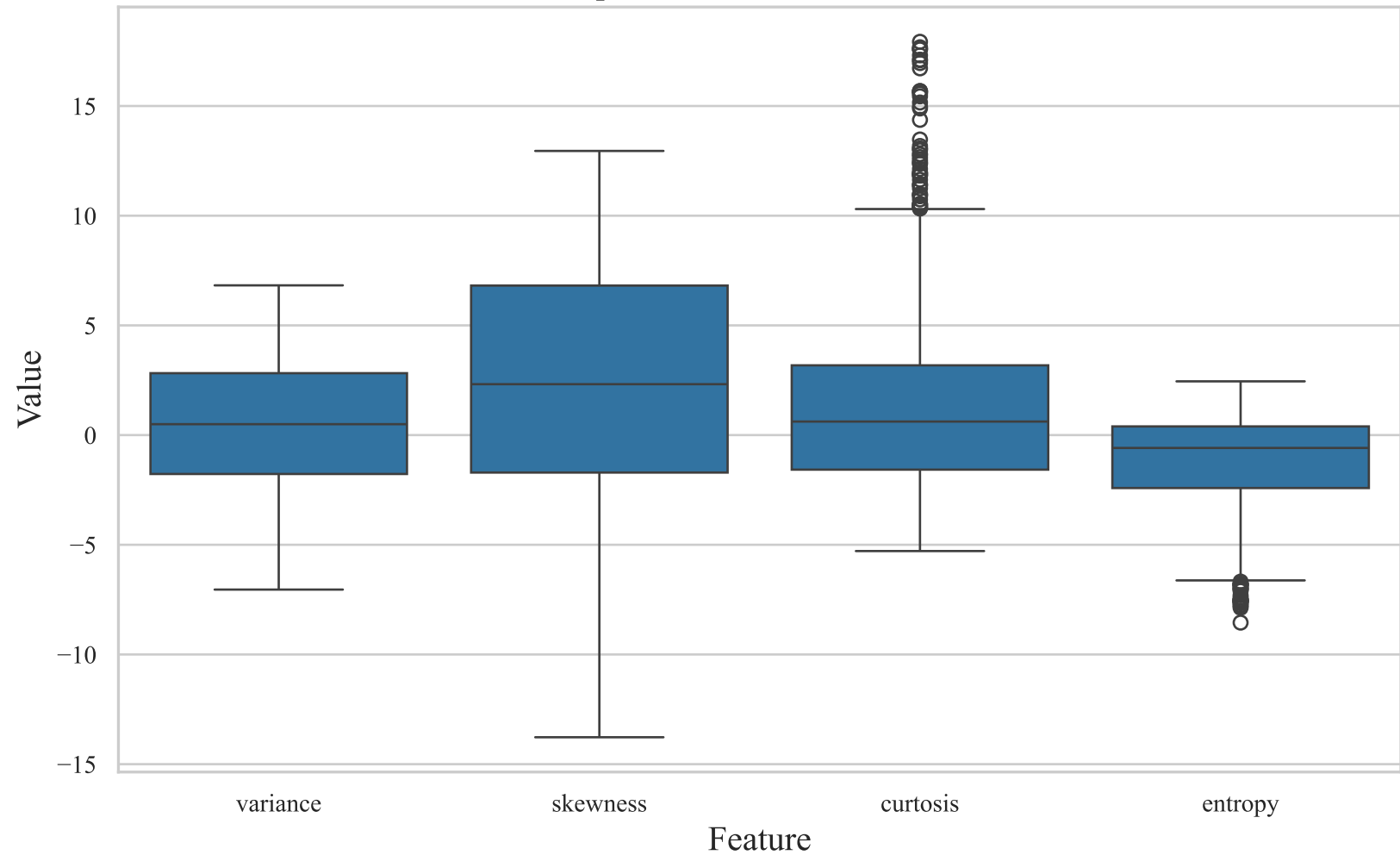
Boxplots of Numerical Features
